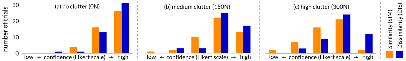
Figure 9: Confidence of marked clusters (Task 2). Participants have higher confidence in their cluster selection using dissimilarity ordering.
