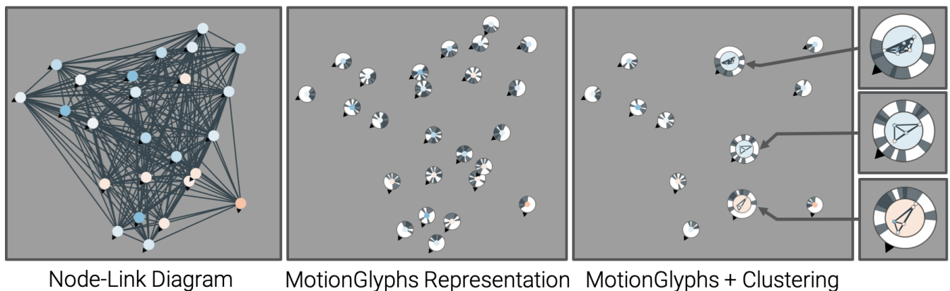
Figure 1: MotionGlyphs allows biologists to visually explore and abstract dense spatio-temporal network data in collective animal behavior. The figure presents the same time instance of golden shiner fish data in a node-link diagram (left), MotionGlyphs representation (middle), and with additional clustering (right). The color of the movers displays the speed (blue to red), and the links (light blue to dark blue) encode the similarity between movement properties (direction, speed, distance to each other). The example above shows how MotionGlyphs abstract relationships and aggregate movers into groups to reduce visual clutter and highlight different group structures.
