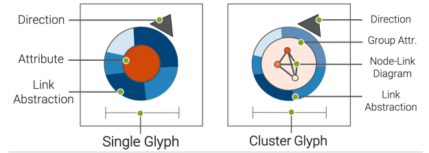
Figure 4: Glyph for single movers (left) and for group of movers (right). The inner-circle display attributes (e.g., speed) and the outer-ring abstracted links to other movers.
