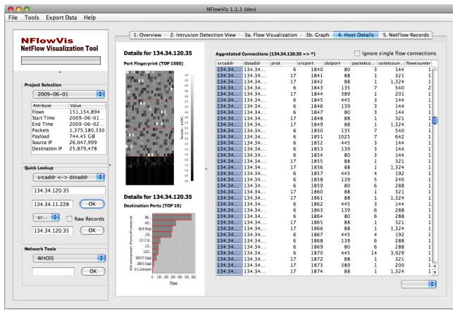
(a) Host details view
