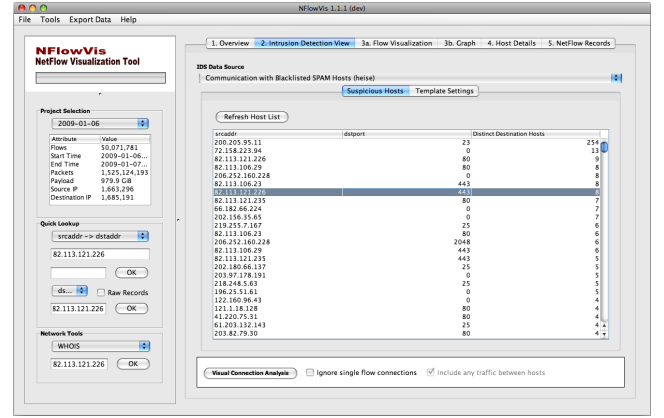
Figure 3: Intrusion detection view
