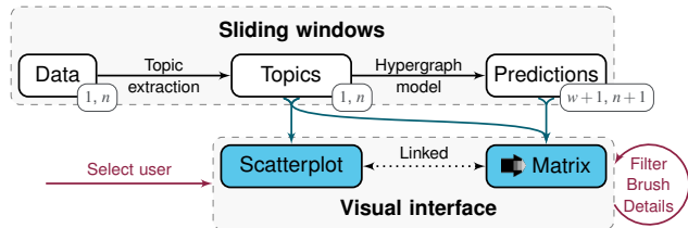
Figure 1: Our visual analytics framework integrates temporal hypergraph predictions by joining multiple (n - w) sliding windows of size w in arrow glyphs in the matrix view (See Sect. 3). The top row shows the main data flow, while the bottom row depicts the domain expert’s workflow with the visual analytics system (red arrows). Petrol colored arrows between rows show how data is mapped to the visual interface.
