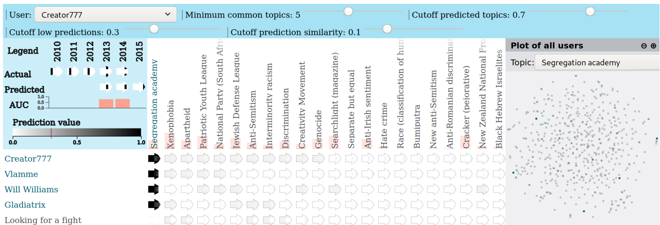
Figure 2: Overview on the visual interface. At the top there is the main filter panel (blue background) including controls to select the user to focus on, and sliders to set cutoff values for filtering the elements displayed in the matrix view. Below there is the matrix view on the left hand side including the glyph legend (light blue background). The arrow shape eases understanding by explicating time direction, and by separating glyphs. Placing predictions in the middle increases the visual saliency of misses. On the right hand side, the scatterplot view offers an overview on all users (gray background). Topic Segregation academy is highlighted, hence only the arrow glyphs for this topic are shown in the matrix, and users that are part of this hyperedge are colored in both views. Bars in the background of topic labels depict how popular each topic is. The solid dots in the scatter plot represent those users that are currently shown in the matrix view. On demand additional details are displayed as tooltips.
