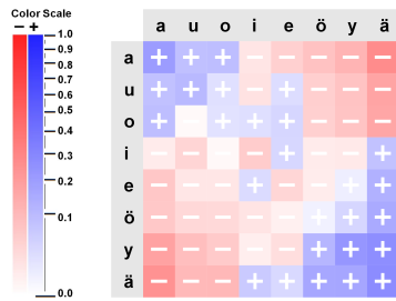
Figure 2: The visualization represents the \phi matrix for the Finnish Bible. In this case the “+” and “-” symbols provide a redundant mapping. Now, blocks of vowels that belong together can clearly be seen. As before, {a,u,o} build one block, {ö,y,ä} another independent block, and {i,e} cannot unambiguously be assigned to any of them. In fact, this conforms nicely to the categorization linguists have for Finnish vowels: {a,u,o} are back vowels, {ö,y,ä} are front vowels, and {i,e} are neutral vowels, which explains that they do not adhere to one of the blocks.
