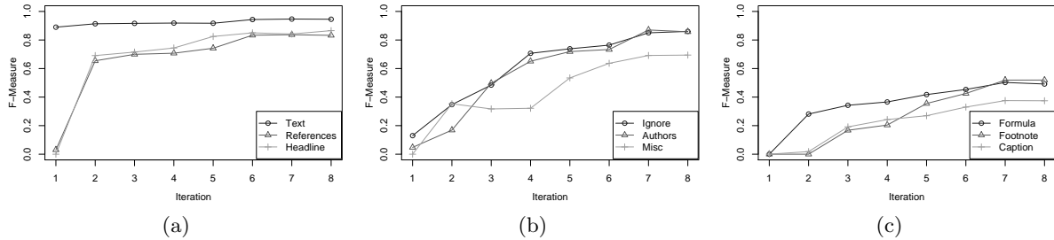
Figure 3: Average F-measure of the structure analysis in the different reference data iterations.
